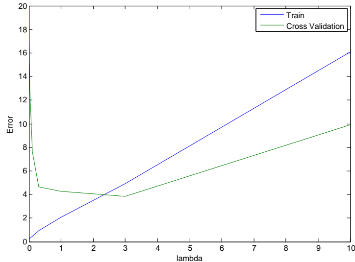
Figure 9: Selecting \lambda using a cross validation set
